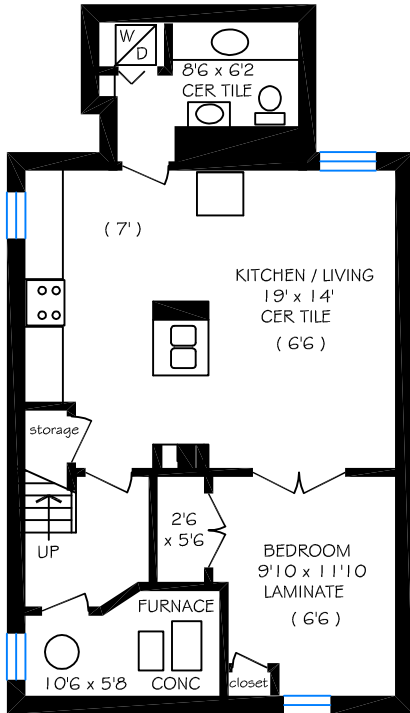
BASEMENT FLOOR = 770 SQ FT
